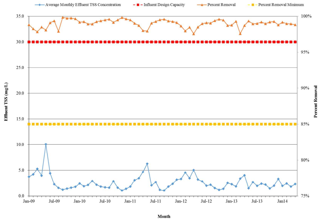
Effluent TSS Concentration and Percent Removal Jan 2009 through Apr 2014
