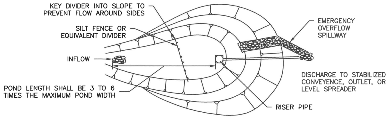
PLAN VIEW
