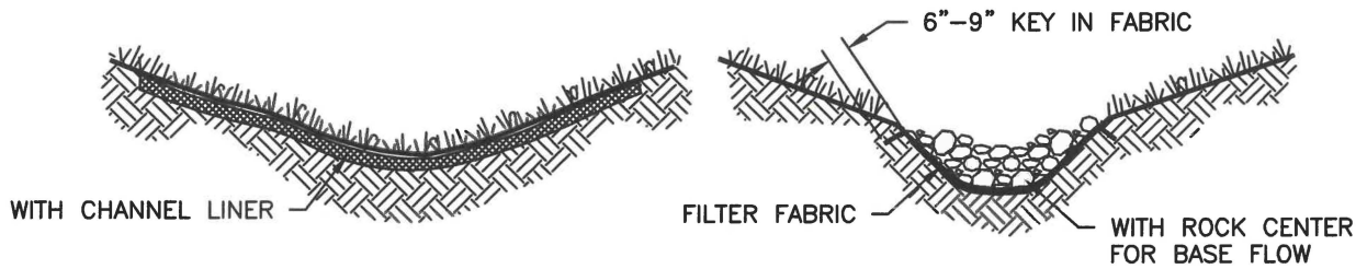
TYPICAL PARABOLIC CHANNEL CROSS-SECTION
