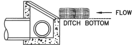
DITCH INLET
