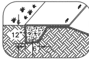
TERMINAL SLOPE & CHANNEL ANCHOR TRENCH
