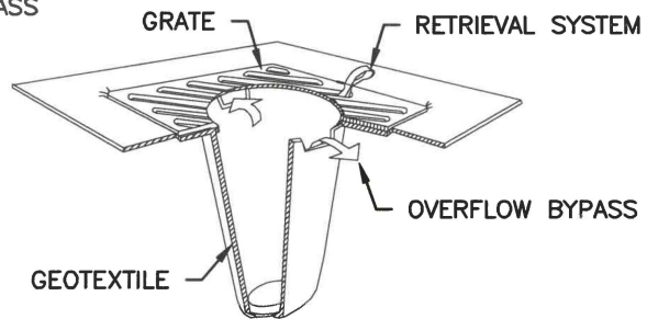
ISOMETRIC VIEW
