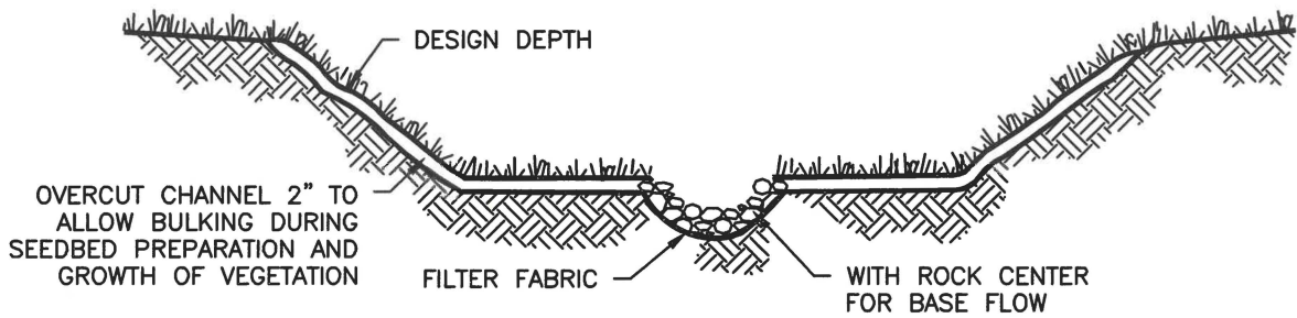
TYPICAL TRAPEZOIDAL CHANNEL CROSS-SECTION
