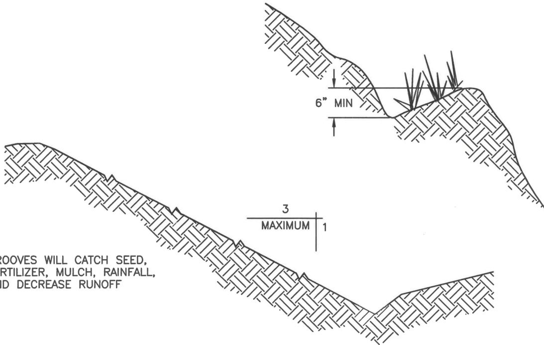
CONTOUR FURROWS
