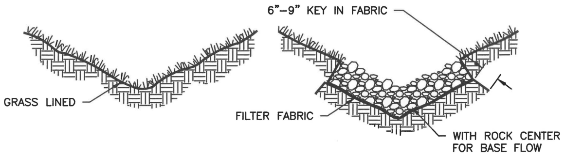
TYPICAL V-SHAPED CHANNEL CROSS-SECTION
